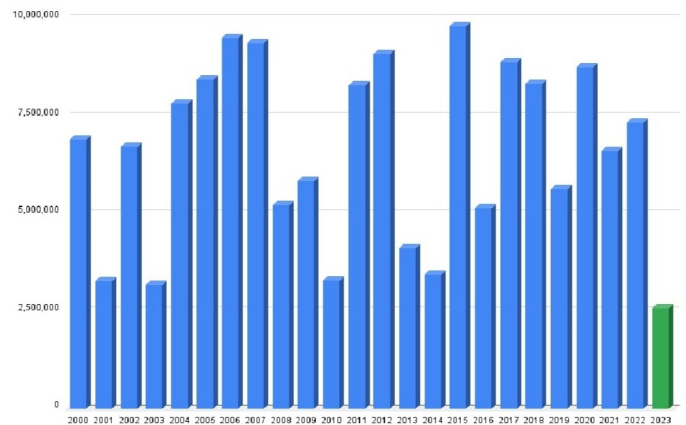
US Forest Fire Burn Acreage Through November 17 https://www.nifc.gov/fire-information/rfm
