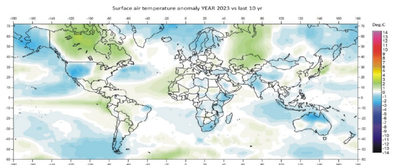
FIGURE 1: Year 2023 surface air temperatures compared to the average for the previous 10 years. Green-yellow-red colours indicate areas with higher temperature than the average, while blue colours indicate lower than average temperatures. Data source: Remote Sensed Surface Temperature Anomaly, AIRS/Aqua L3 Monthly Standard Physical Retrieval 1-degree x 1-degree V006 ( https://airs.jpl.nasa.gov/ ), obtained from the GISS data portal ( https://data.giss.nasa.gov/gistemp/maps/ ).
