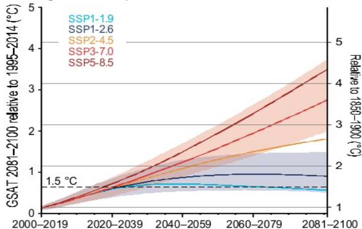
Warming to 2100 depends on the scenario
