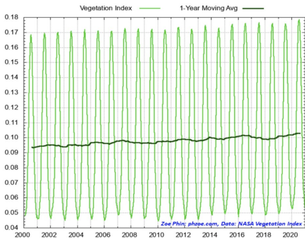
NASA's Vegetation Index has risen from 0.0936 to 0.1029, which is a 9.94% increase. Chart by Zoe Phin
