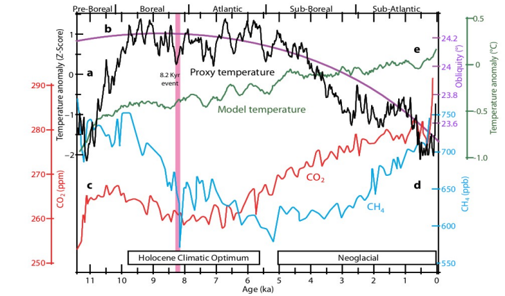
Fig. 4.5 Temperature and greenhouse gases during the Holocene a) Black curve, global temperature reconstruction as in Fig. 4.4b. b) Purple curve, Earth's axis obliquity cycle. c) Red curve, CO 2 levels as measured in Epica Dome C (Antarctica) ice core, reported in Monnin et al. (2004). d) Blue curve, methane levels as measured in GRIP, GISP2, and NEMO (Greenland) ice cores as reported by Kobashi et al. (2007). Notice the great effect of the 8.2 kyr event on methane concentrations. e) Green curve, simulated global temperature from an ensemble of three models (CCSM3, FAMOUS, and LOVECLIM) from Liu et al. (2014), show the inability of general climate models to replicate the Holocene general temperature downward trend. Vertical bar, 8.2 kyr BP ACE. Major Holocene climatic periods are indicated.
