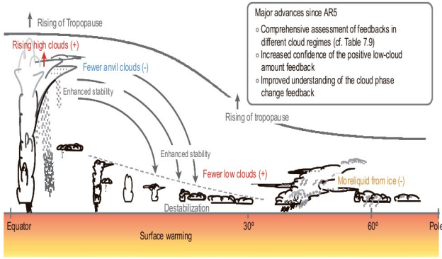
Figure 7.9 | Schematic cross section of diverse cloud responses to surface warming from the tropics to polar regions. Thick solid and dashed curves indicate the tropopause and the subtropical inversion layer in the current climate, respectively. Thin grey text and arrows represent robust responses in the thermodynamic structure to greenhouse warming, of relevance to cloud changes. Text and arrows in red, orange and green show the major cloud responses assessed with high, medium and low confidence, respectively, and the sign of their feedbacks to the surface warming is indicated in the parenthesis. Major advances since AR5 are listed in the box. Figure adapted from Boucher et al. (2013).
