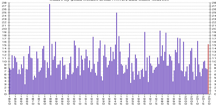
San Diego Annual Rainfall by Calendar Year
