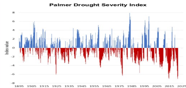
The Palmer Drought Severity Index measures the relative dryness of a region by incorporating readily available temperature, precipitation, and soil moisture data. Between 2010 and 2021, there were 48 months when index values were at or below -3 (representing severe drought), including eight months with values below -6 (representing very extreme drought).
