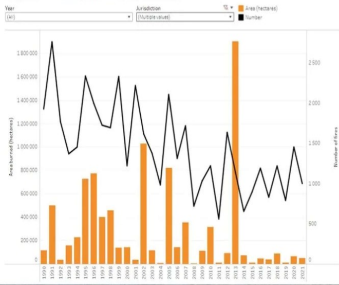
Forest fires in Quebec. Source: NFDP
