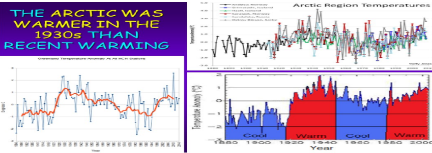
Figure 9. Arctic temperatures were warmer in the 1930s than today. The graph on the left shows temperatures in Greenland from 1894 to 2014 (high temperatures in left center during the 1930s) were warmer than today (right side). Upper right graph is Arctic temperature from Iceland, Russia, and Norway showing that the 1930s were warmer than recent decades. Lower right shows Arctic temperatures from 1880 to 2000 for 70–90° latitude. Note that the 1920s and 1930s were warmer than 2000. (Easterbrook, 2016).
