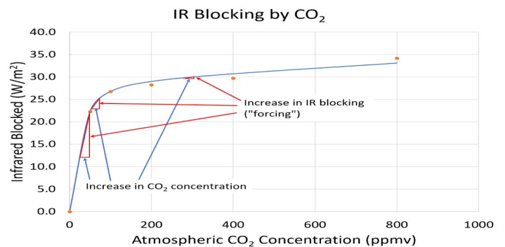
Figure 6: IR blocking for CO2 concentrations from 0 to 800 ppmv. Given an increase in the CO2 concentration, the effect decreases as the amount of atmospheric CO2 increases.
