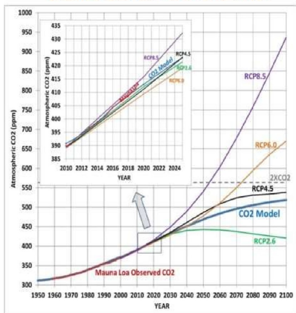
Model Projection of Atmospheric CO2 to 2100
