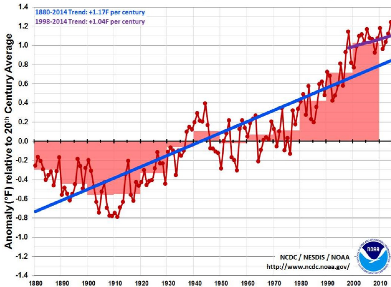
Annual Global Temperature (Combined Land & Ocean)
