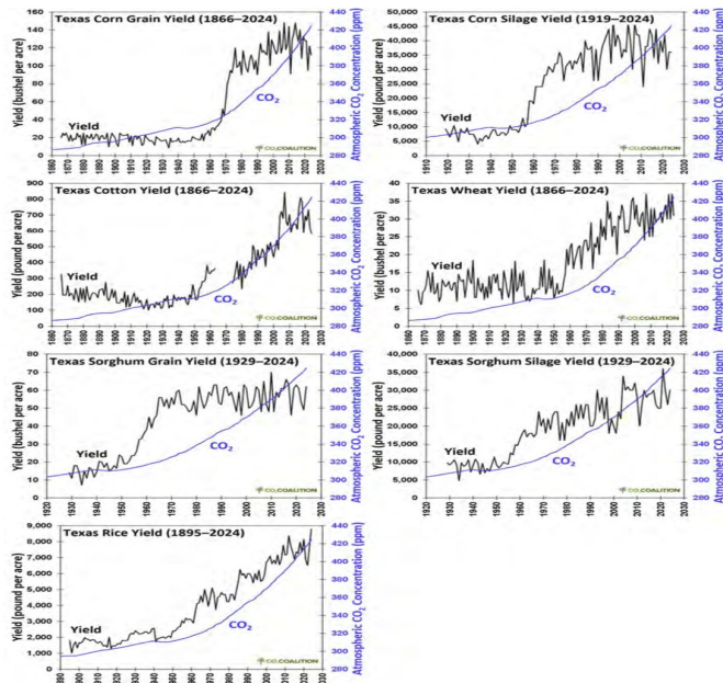
Figure 17: Primary Crop Yields in Texas, Plotted With the Atmospheric CO 2 Concentration. Crop yield: USDA National Agricultural Statistics Service (2025), CO 2 concentration (1958 and prior): NASA Goddard Institute for Space Studies (2018), CO 2 concentration (1959 onward): Lan and Keeling (2025) (NOAA)
