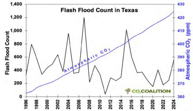
Figure 9: Annual Reported Number of Flash Floods in Texas, Plotted With the Atmospheric CO 2 Concentration. Flash floods: NOAA National Centers for Environmental Information (2025c), CO 2 concentration (1958 and prior): NASA Goddard Institute for Space Studies (2018), CO 2 concentration (1959 onward): Lan and Keeling (2025) (NOAA)
