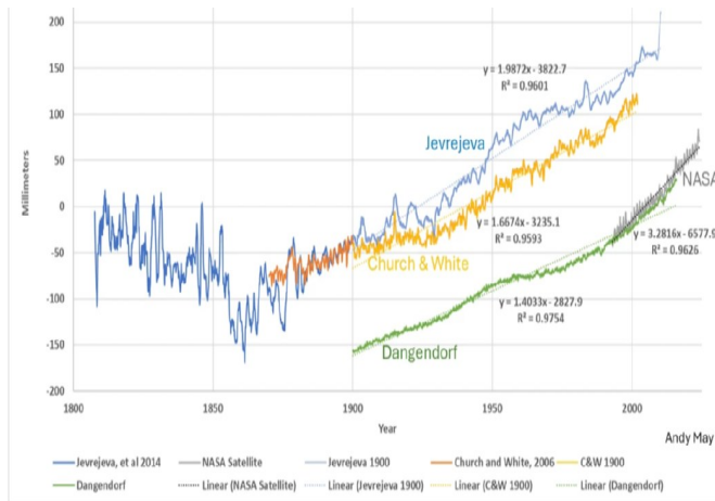
Figure 2. A Comparison of various estimates of the rate of global sea level rise. The Jevrejeva and Church & White estimates are from tide gauges, the NASA estimate (Beckley, Callahan, Hancock, Mitchum, & Ray, 2017) is from satellite measurements, and the Dangendorf record is a complex hybrid.
