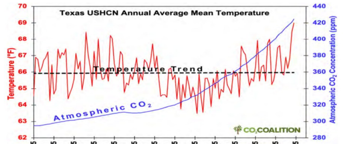
Figure 3: USHCN Corrected Annual Average Mean Temperature in Texas, Plotted With the Atmospheric CO 2 Concentration. Temperature: NOAA National Centers for Environmental Information (2025d), CO 2 concentration (1958 and prior): NASA Goddard Institute for Space Studies (2018), CO 2 concentration (1959 onward): Lan and Keeling (2025) (NOAA)
