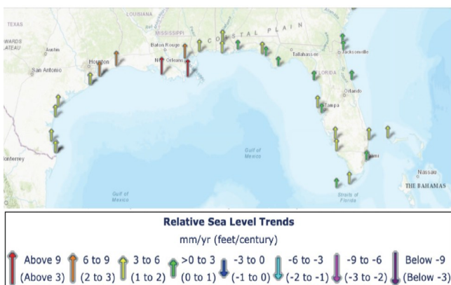
Figure 13. Relative change in sea level at various tide gauge stations along the southeastern US coastline (NOAA). These values essentially provide the net change when considering changes in land elevation as well as sea level.
