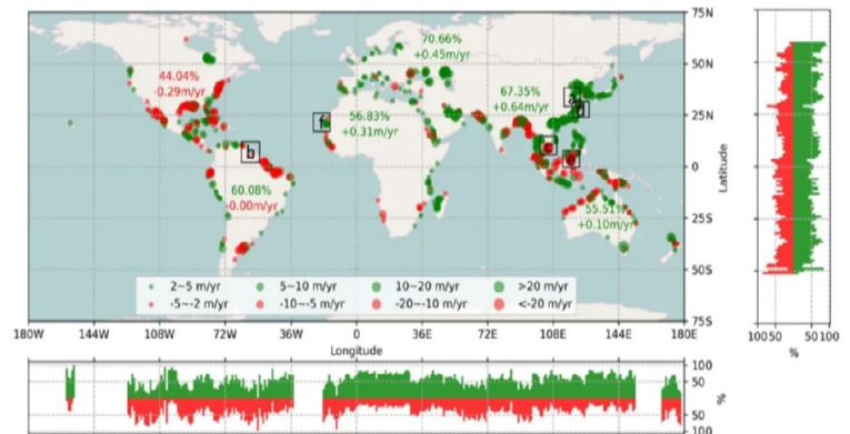
At almost all latitudes and longitudes landification is winning out over erosion and SLR. Figure 9 from Mao et al. 2021.
