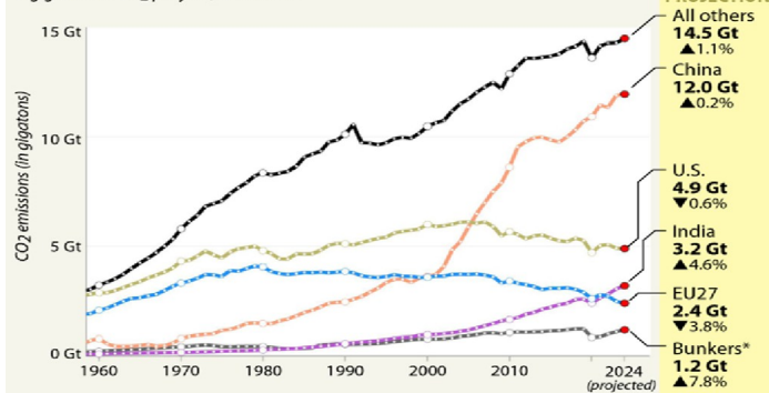
ANNUAL FOSSIL CO 2 EMISSIONS In gigatons of CO 2 per year, 1960-2024
