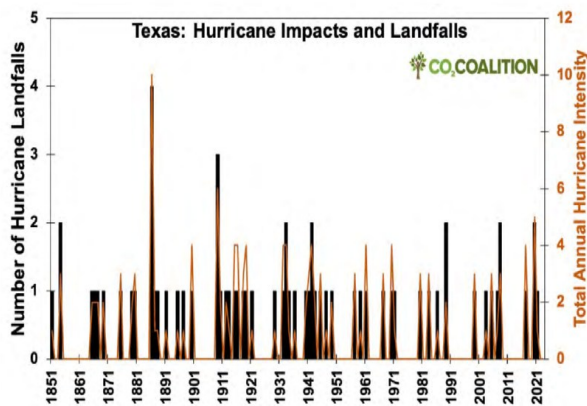
Figure 13: Annual Number and Total Intensities of Hurricane Impacts and Landfalls in Texas. NOAA Atlantic Oceanographic & Meteorological Laboratory (2024)
