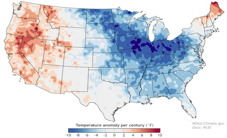
Average temperature trends, February 1987-2016 (30 years)
