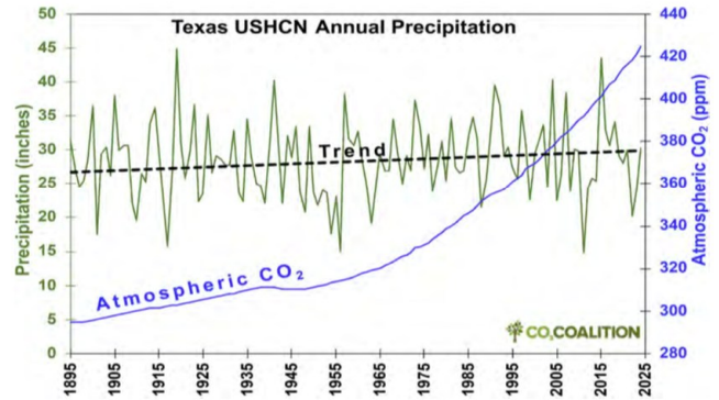
Figure 7: Annual Precipitation in Texas, Plotted With the Atmospheric CO 2 Concentration. Precipitation: NOAA National Centers for Environmental Information (2025d), CO 2 concentration (1958 and prior): NASA Goddard Institute for Space Studies (2018), CO 2 concentration (1959 onward): Lan and Keeling (2025) (NOAA)
